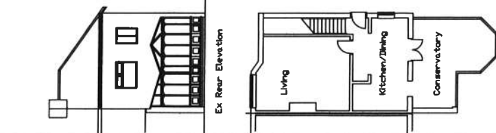
Ex Ground Floor
